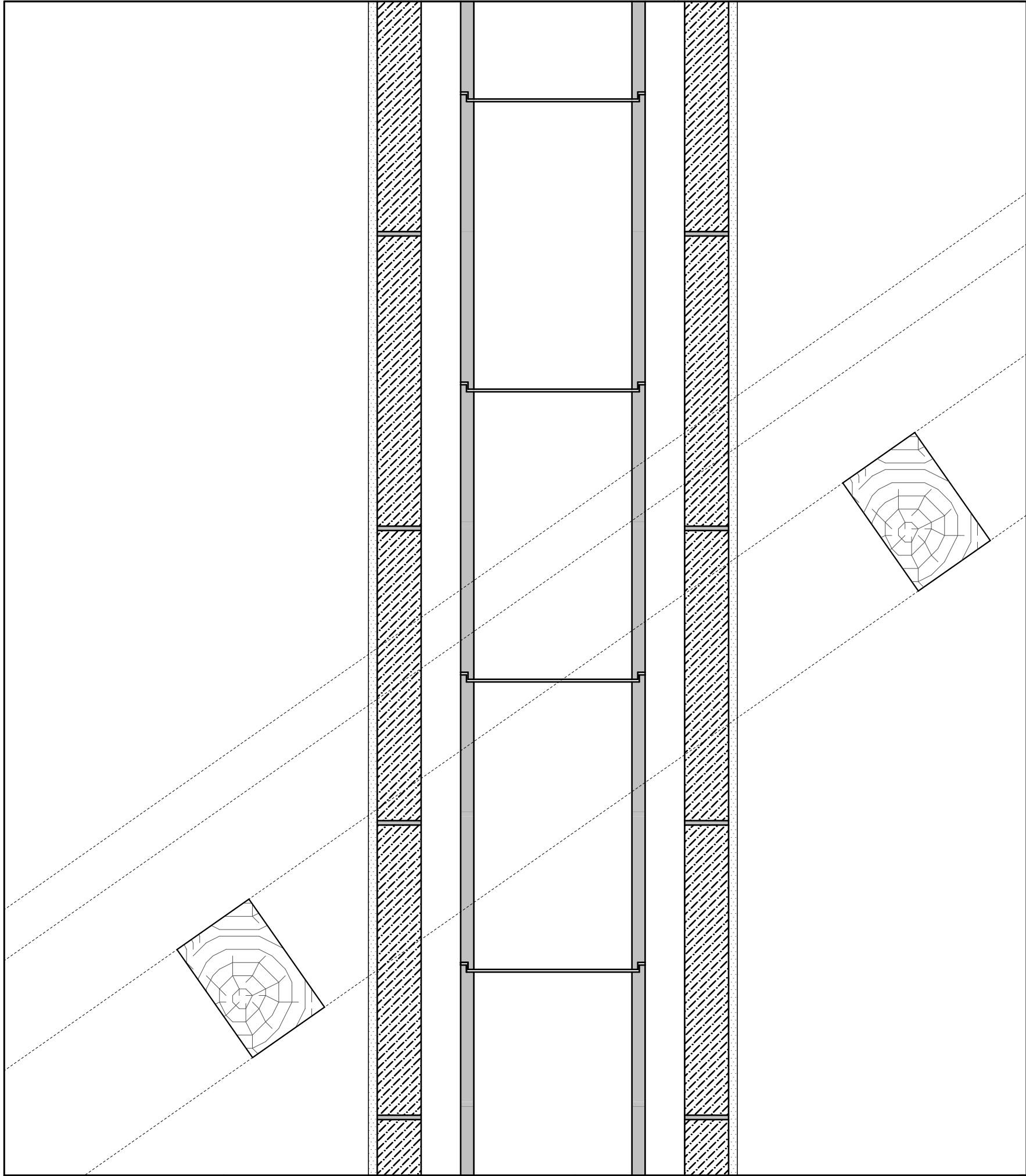
DOUBLE SEAM METAL ROOF CLADDING RIDGE VENTILATION (PRACTICE)
