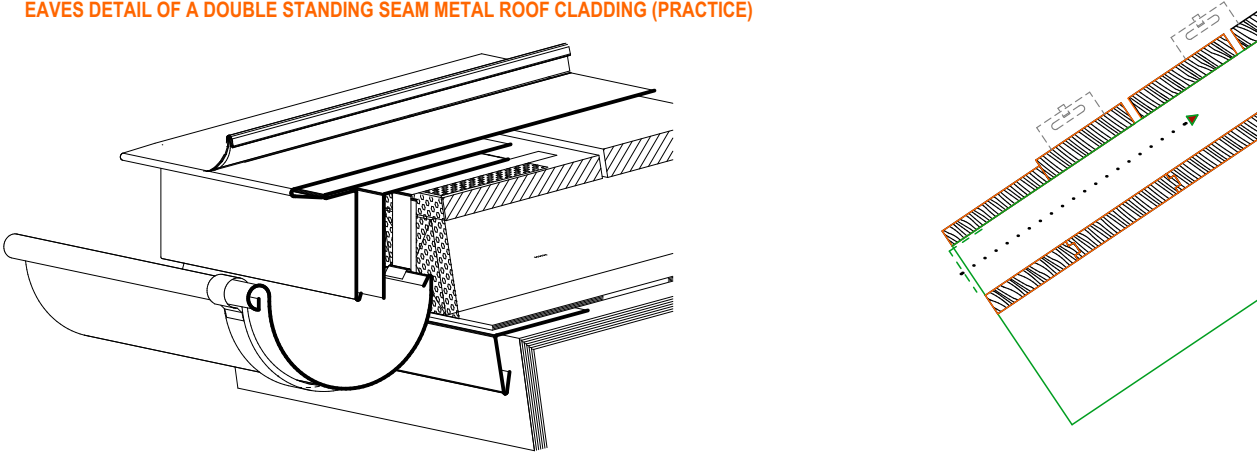
EAVES DETAIL OF A DOUBLE STANDING SEAM METAL ROOF CLADDING (PRACTICE)
