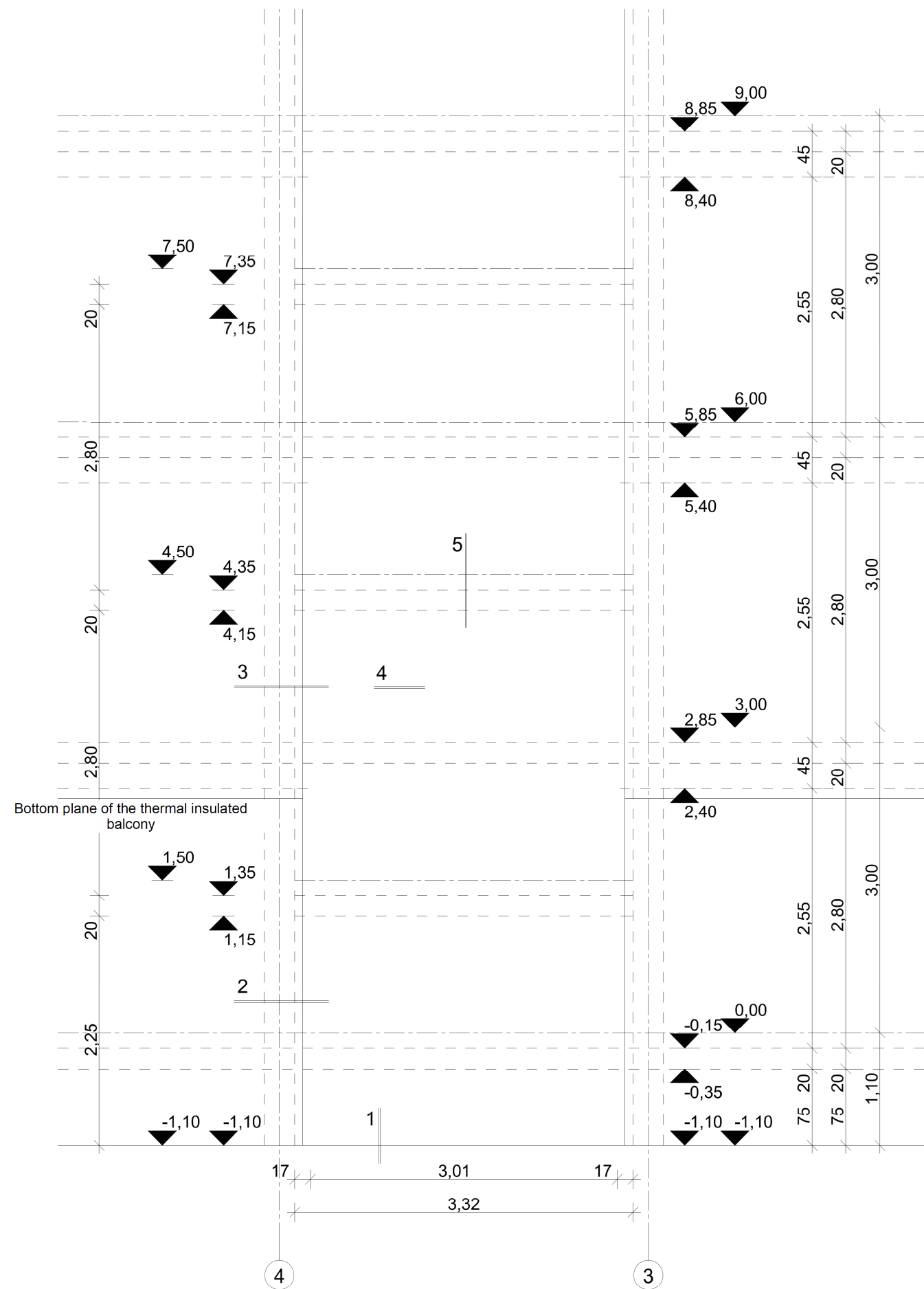
Curtain wall of the staircase - View 1:50
