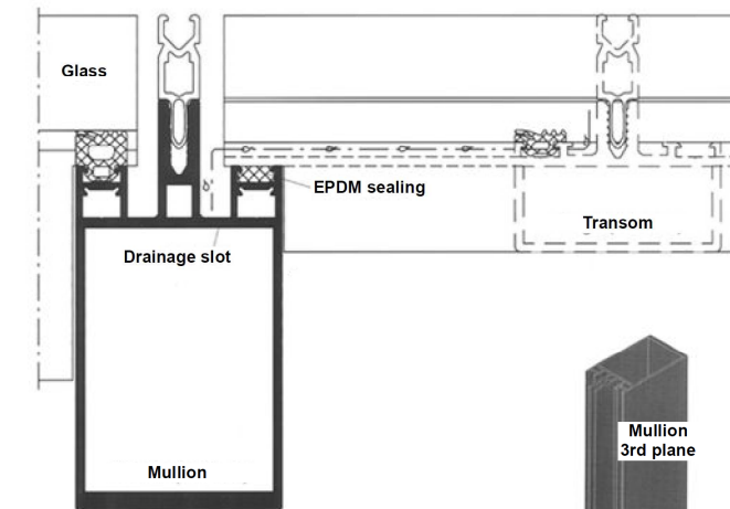
Connection of the mullions and the transoms Drainage system
