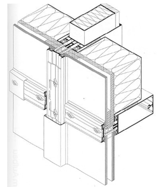
Axonometric view of the glazing and glazed panels
