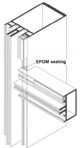
Connection of the mullions and the transoms Drainage system
