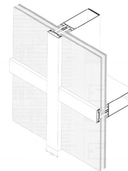
Axonometric view of the glazing and glazed panels
