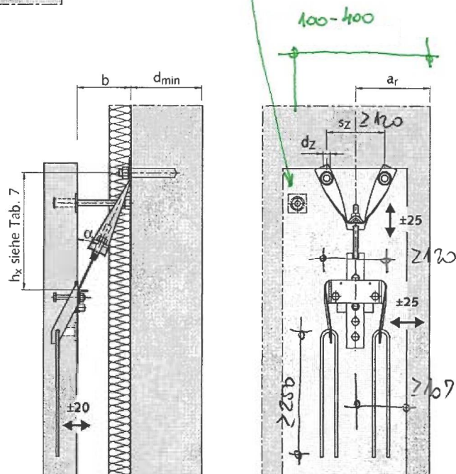
3. WITH DÜBELTYPE FIXTURE
