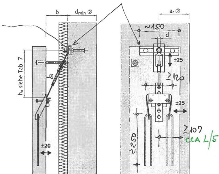
2. WITH "C" RAIL IN THE CONCRETE
