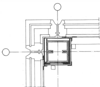
FLOOR PLAN DETAIL
